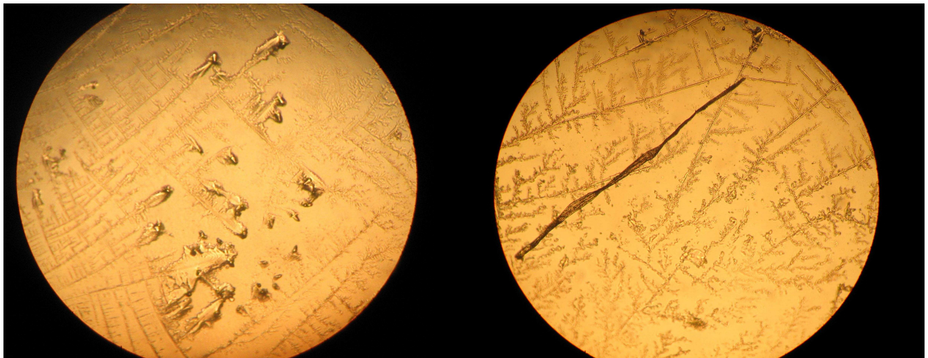
Figure 4. Dry microscope slide mounts of hot water shower samples.
